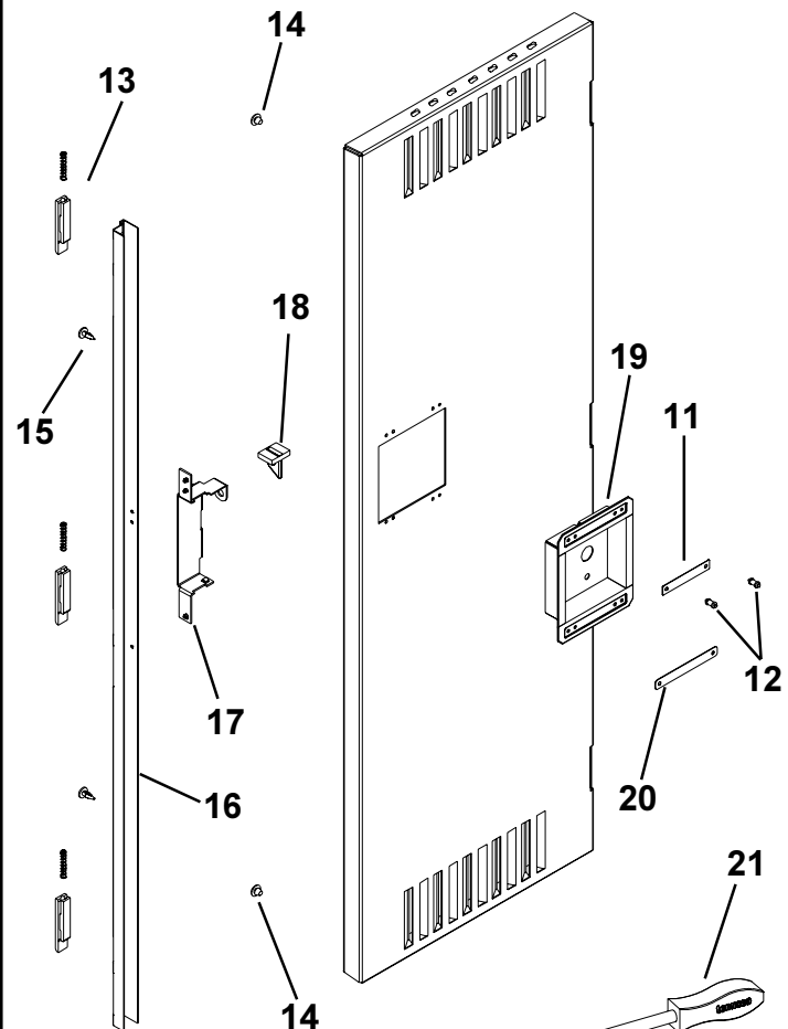
DOOR-LOCK DETAIL
