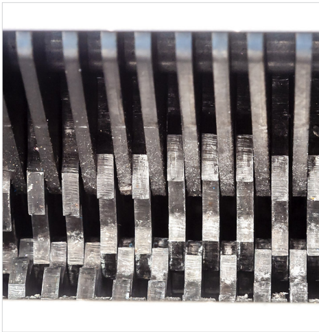
Heavy-duty cutting cylinders are designed for high-volume shredding.
