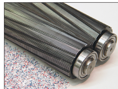
Dahle High Security cutting cylinders reduce a sheet of paper to over 15,500 pieces.
